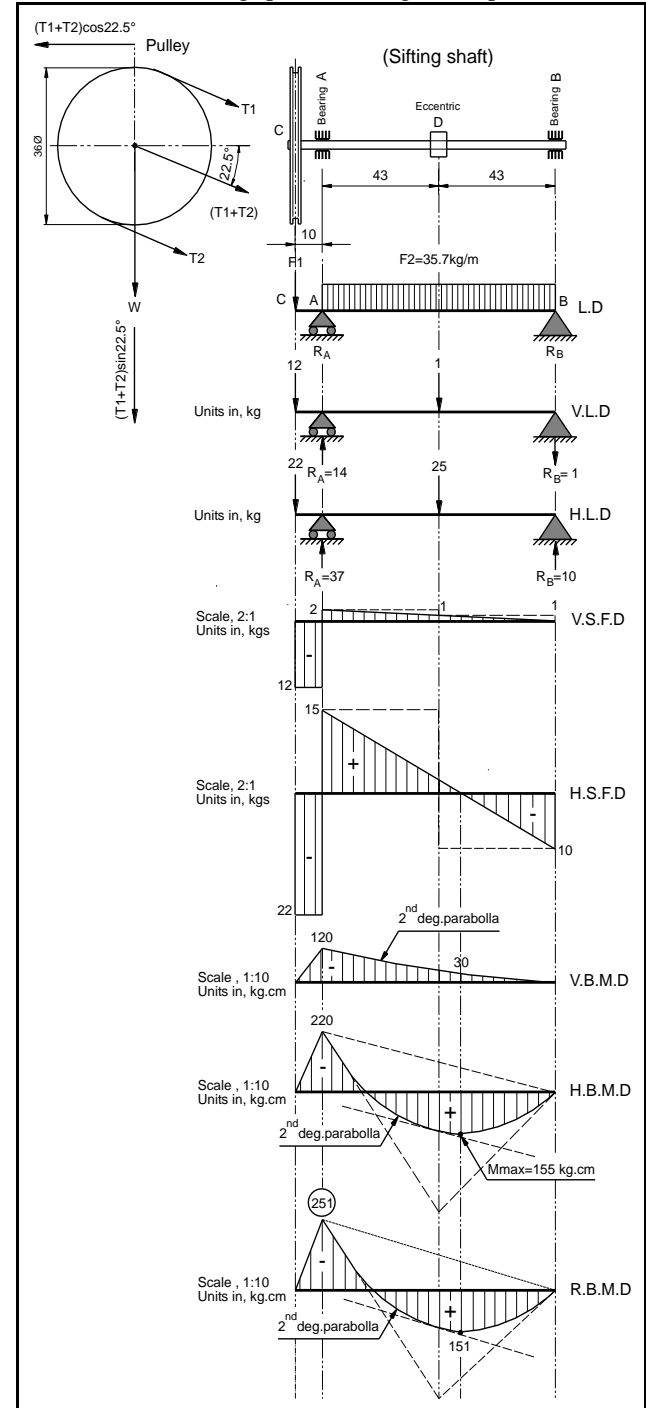
Fig.(2.3): Stress analysis on sifting shaft.
