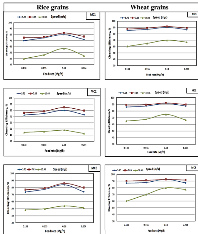
Fig (3.2): Effect of feeding rate on cleaning efficiency at different grain moisture contents and different sieve speeds for rice and wheat grains.
