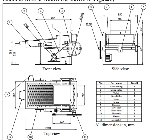
Fig.(2.1): An engineering drawing of the manufactured sifting machine.
