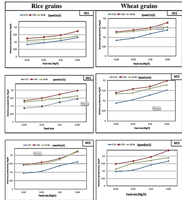
Fig.(3.1): Effect of feeding rate on machine productivity at different grain moisture contents and different sieve speeds for rice and wheat grains.
