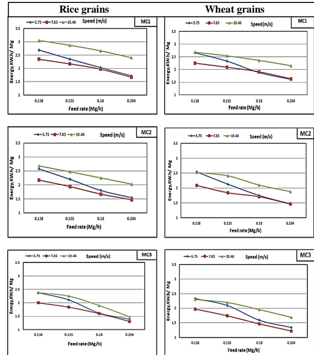
Fig.(3.3): Effect of feeding rate on specific energy consumption at different grain moisture contents and different sieve speeds for rice and wheat.
