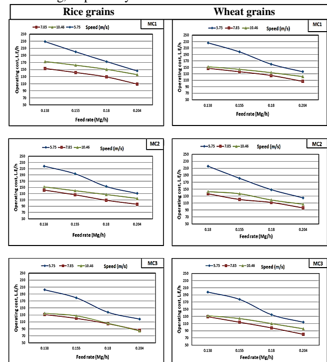
Fig.(3.4): Effect of feeding rate on operating cost at different grain moisture contents and different sieve speeds for rice and wheat grains.
