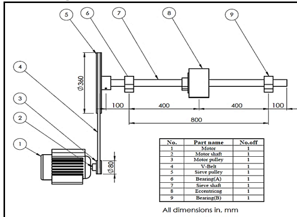
Fig.(2.2): Power transmission from electric motor to cleaning sieve.
